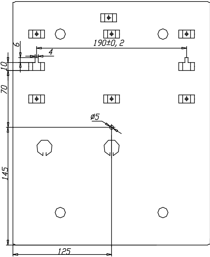
Mounting Dimensions
