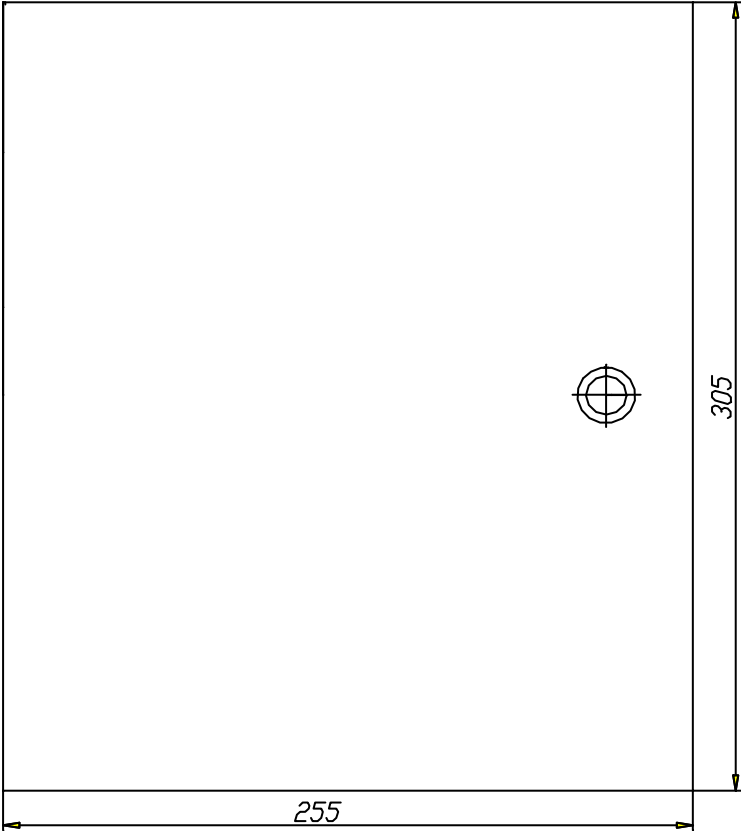
Mounting Dimensions
